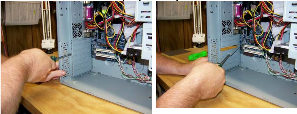
Open slot on back of computer to install card
