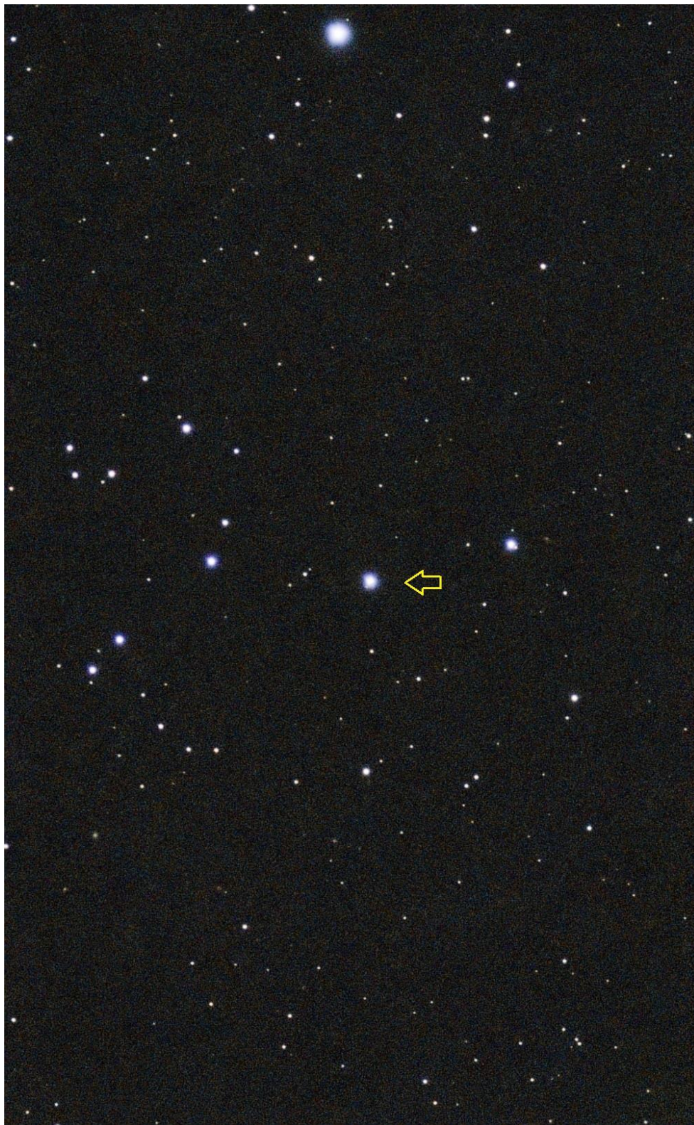
9/20/2026 2:53 am. Pallas to left of yellow arrow. 10 min exposure. Processed and stacked with Siril.
