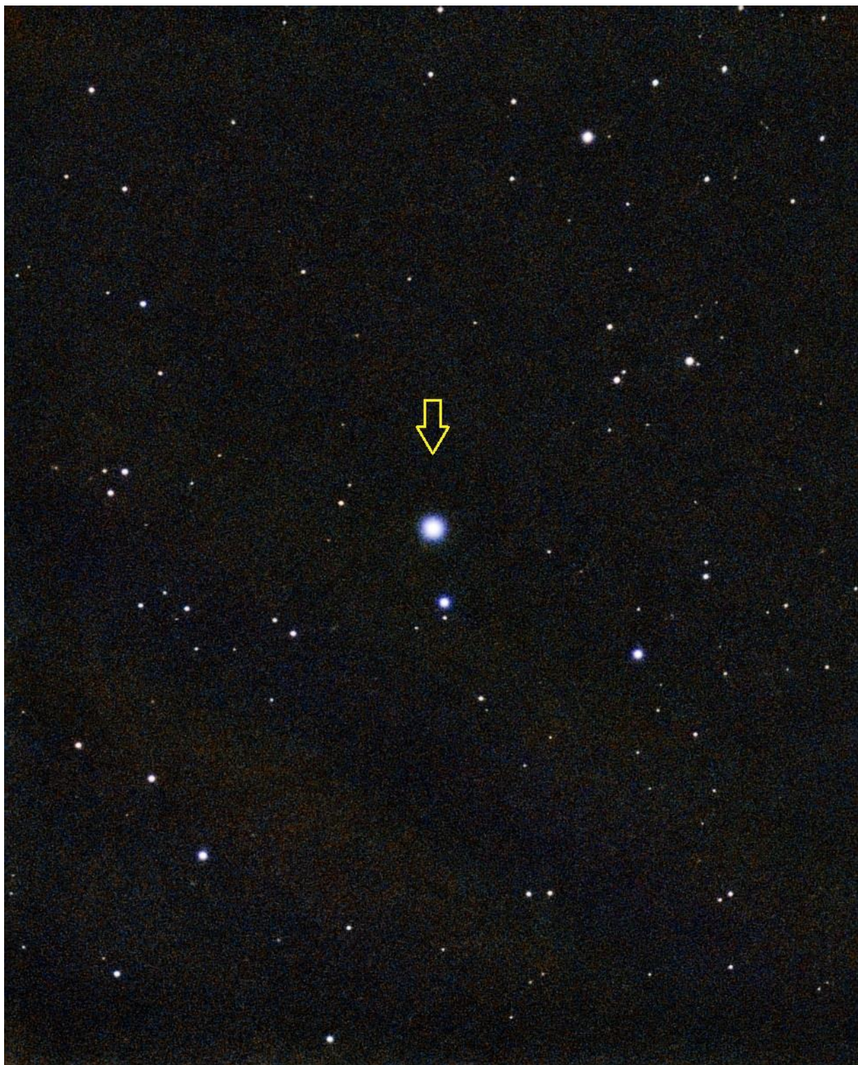
9/27/2026 1:27 am. The arrow shows the location of Pallas. 8 min exposure. Processed and stacked with Siril. Full moon just above this image. Clouds moving in from west at image end.
