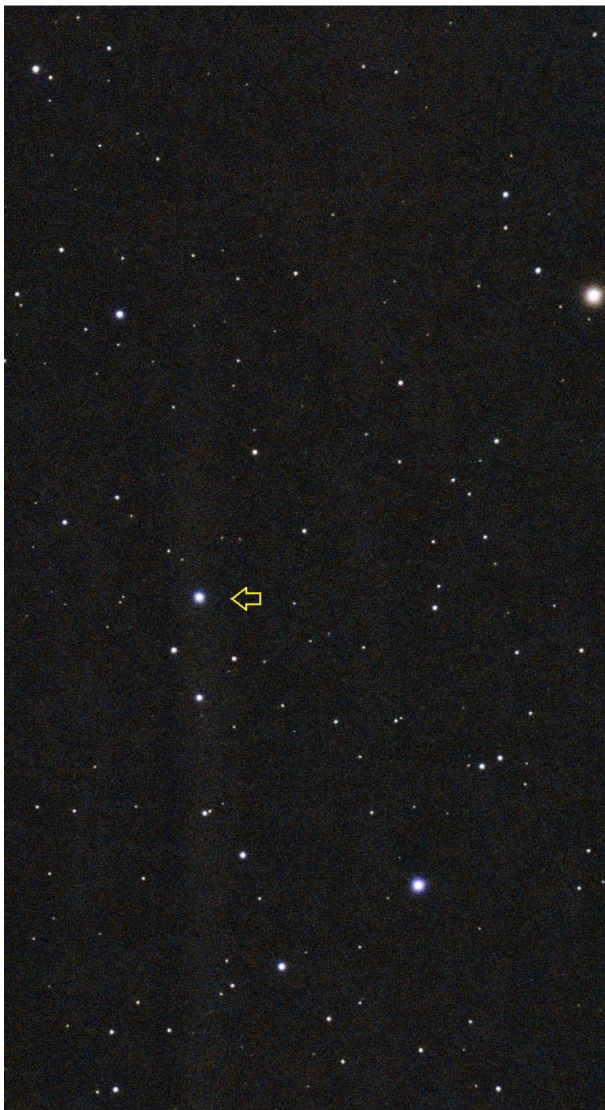
9/26/2026 2:17 am. The arrow shows the location of Pallas. 8 min exposure. Processed and stacked with Siril.
